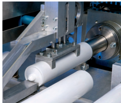
Servo Shuttle
