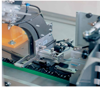
Clip-Nozzle-Station
