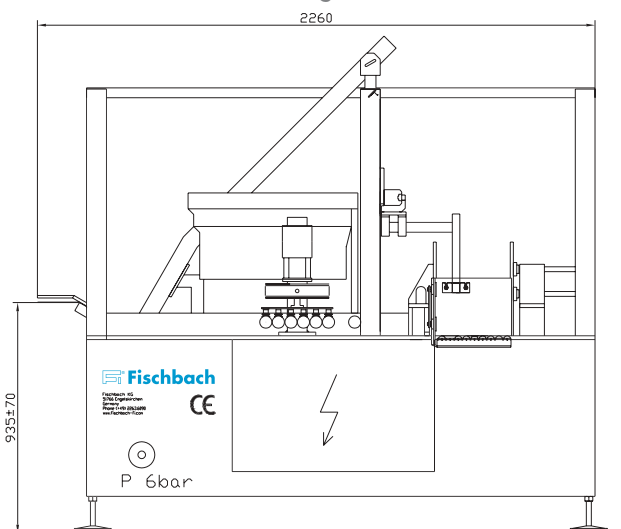
Cartridge Stacker
