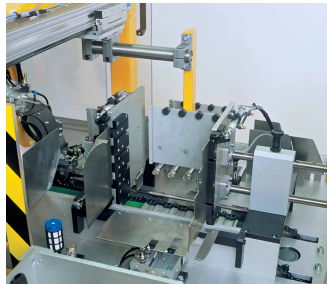
Cartridge Stacker
