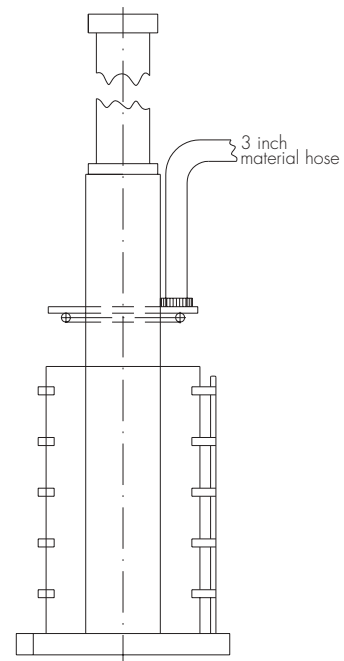
Hydraulic Drum Press FP-1
